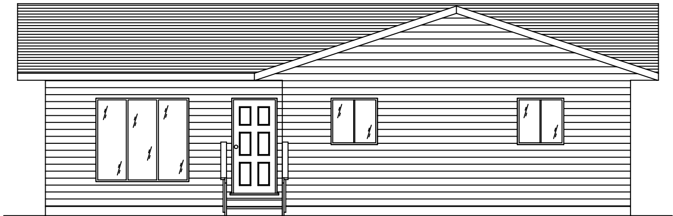
FRONT ELEVATION
